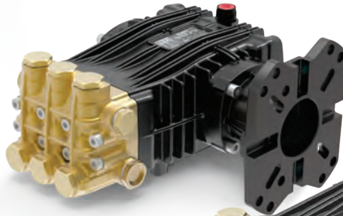
BK SERIES 3.4-5.5 GPM UP TO 4350 PSI Shown with SAE J609-B Flange for 1" Shaft Gas Engines Other drive options available
