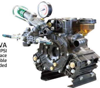
KAPPA 55 VA 15.0 GPM @ 560 PSI Shown with Universal VA Drive Face Other drive options available Regulator / Control Unit is Included
