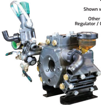
DELTA 75 VA 20.0 GPM @ 560 PSI Shown with Universal VA Drive Face Other drive options available Regulator / Control Unit is Included
