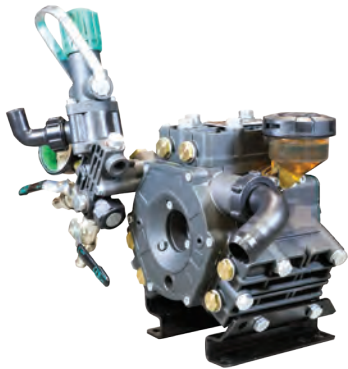
KAPPA 55 VA 15.0 GPM @ 560 PSI Shown with Universal VA Drive Face Other drive options available Regulator / Control Unit is Included
